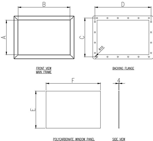
NOTE: 2D drawing is for reference only. See CAD files for sizes and specifications.
