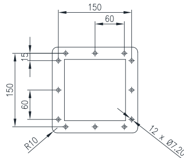
BACKING FLANGE
