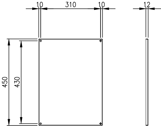
MOUNTING PLATE (PAINTED TO RAL9010)
