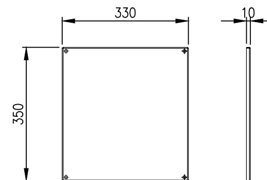
MOUNTING PLATE (PAINTED TO RAL9010)
