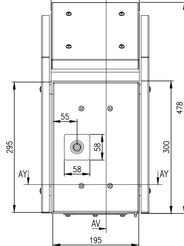
FRONT VIEW
