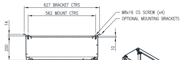
SECTION AW-AW
