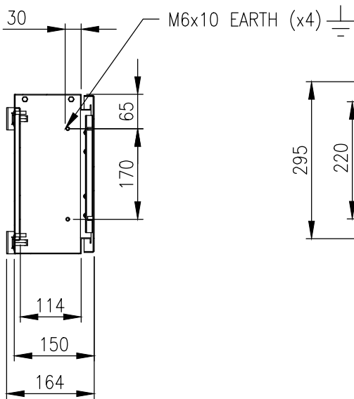
SECTION AW-AW
