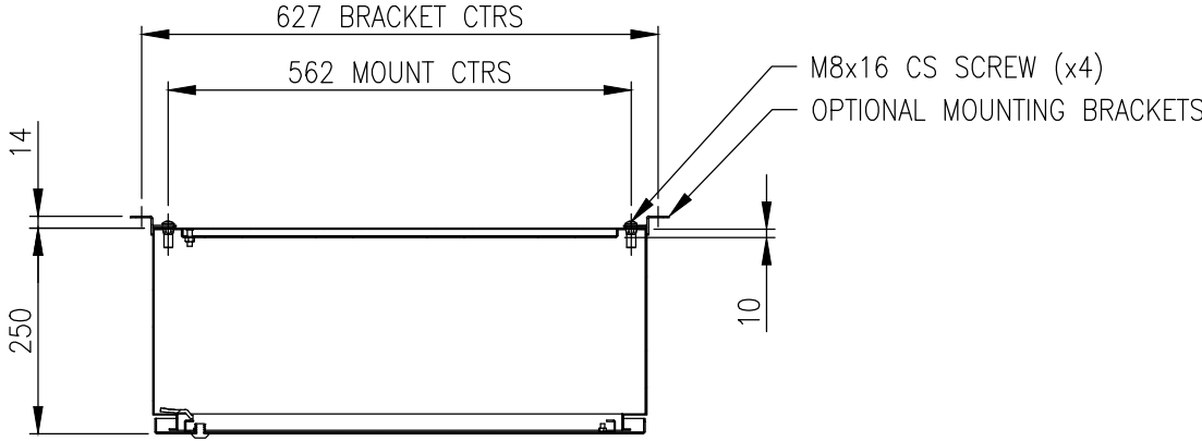
SECTION AW-AW
