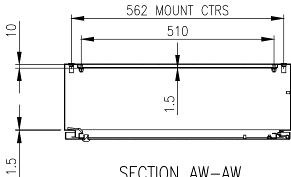
SECTION AW-AW
