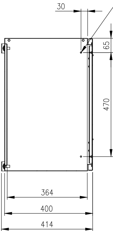
SECTION AY-AW
