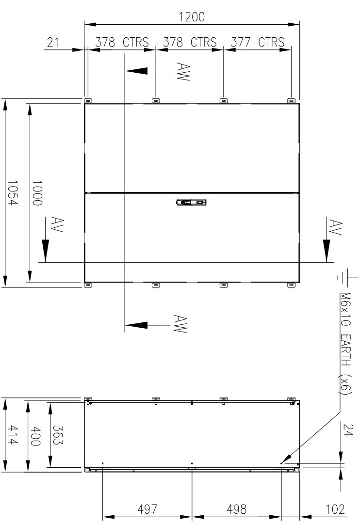
FRONT VIEW
