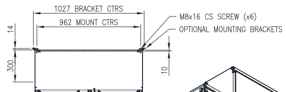
SECTION AW-AW
