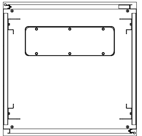
SECTION CC
