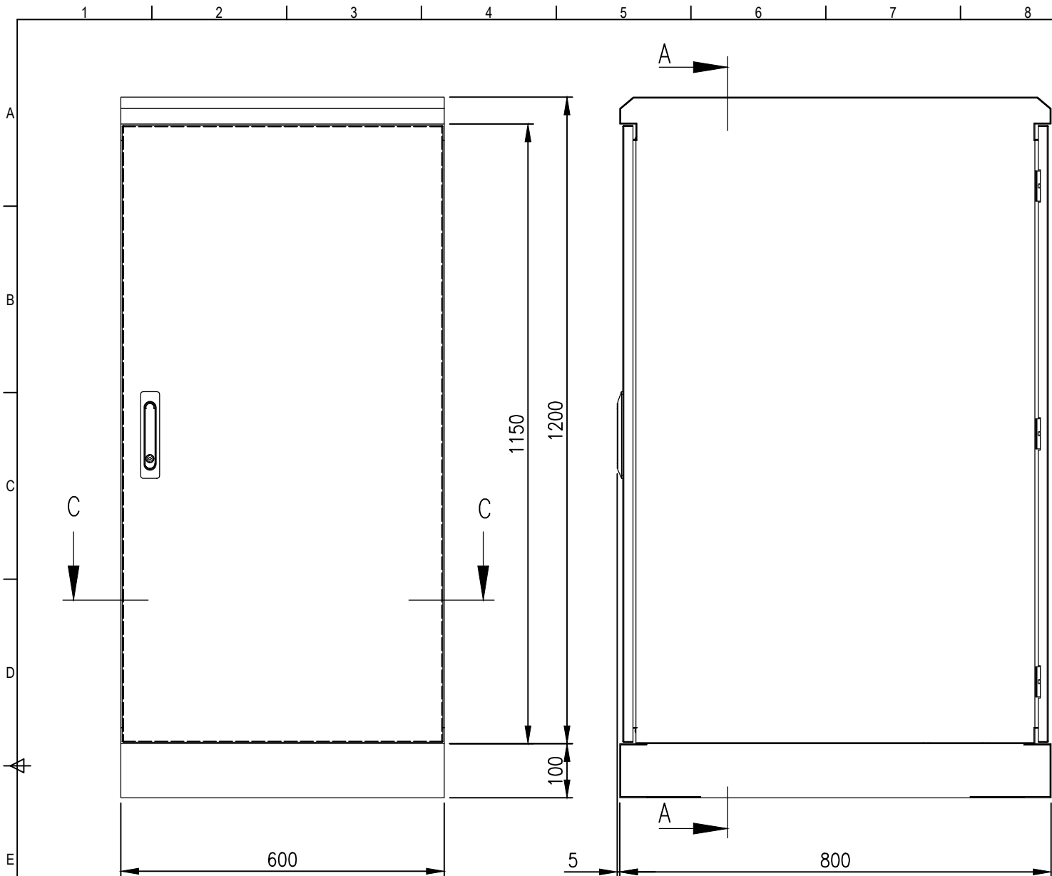
FRONT VIEW
