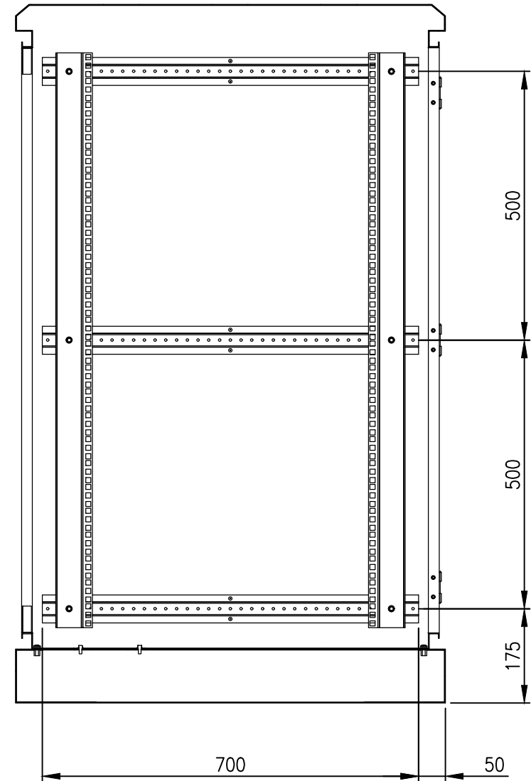
SECTION BB
