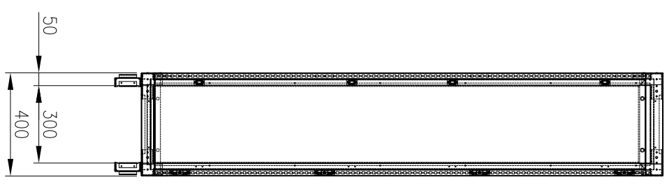
FRONT VIEW (PANELS REMOVED)
