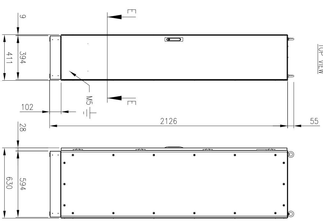
FRONT VIEW (ASSEMBLY)
