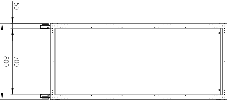
FRONT VIEW (PANELS REMOVED)
