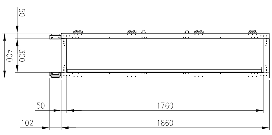
SIDE VIEW (PANELS REMOVED)
