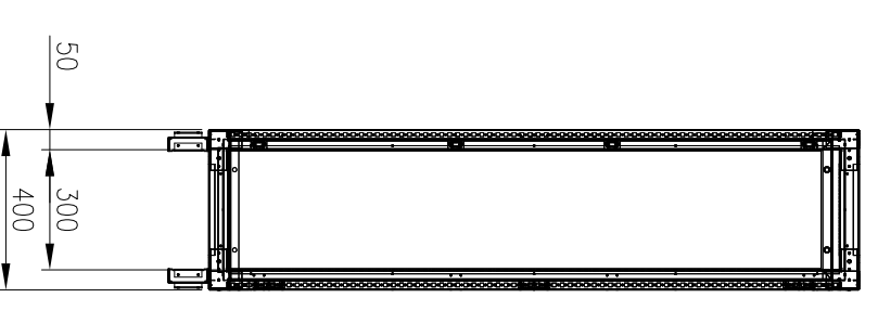
FRONT VIEW (PANELS REMOVED)
