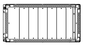
SECTION E-E
