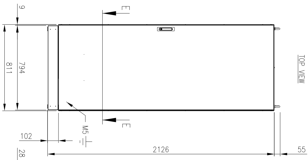
FRONT VIEW (ASSEMBLY)
