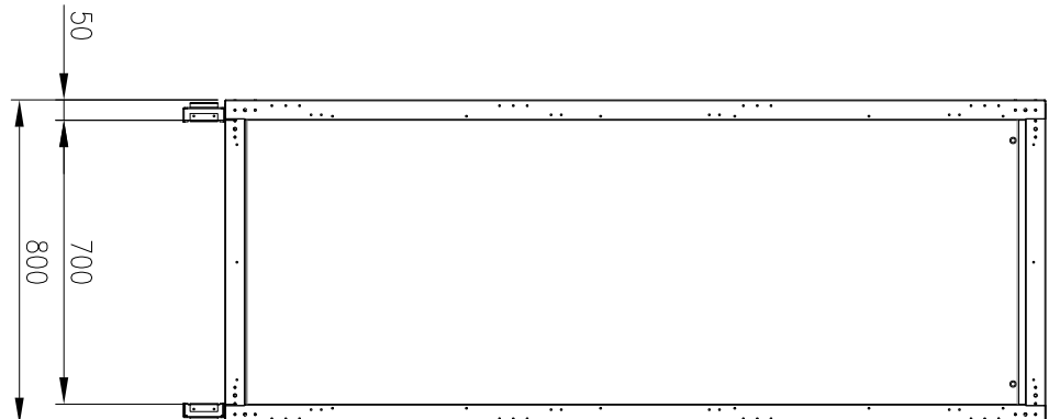
FRONT VIEW (PANELS REMOVED)
