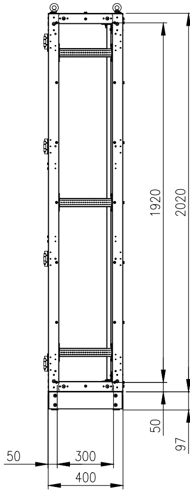
SIDE VIEW (PANELS REMOVED)
