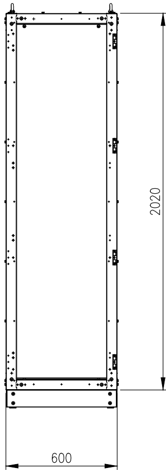
FRONT VIEW (PANELS REMOVED)
