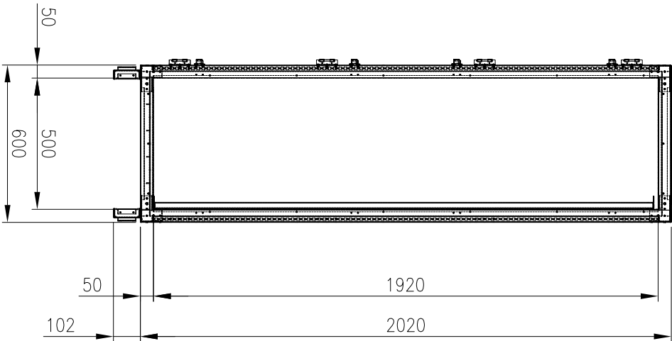
SIDE VIEW (PANELS REMOVED)
