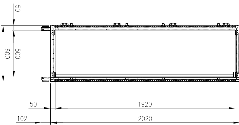
SIDE VIEW (PANELS REMOVED)
