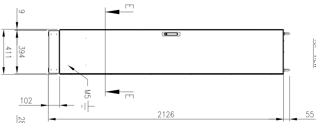
FRONT VIEW (ASSEMBLY)
