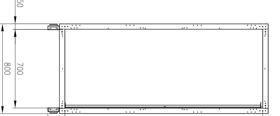
SIDE VIEW (PANELS REMOVED)
