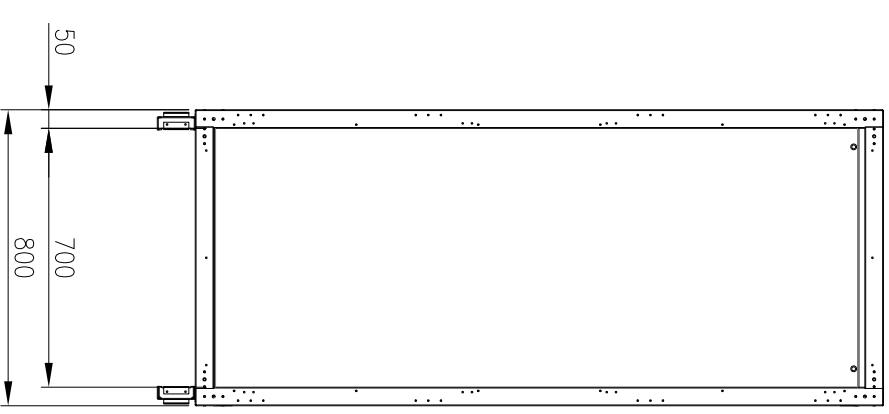
FRONT VIEW (PANELS REMOVED)
