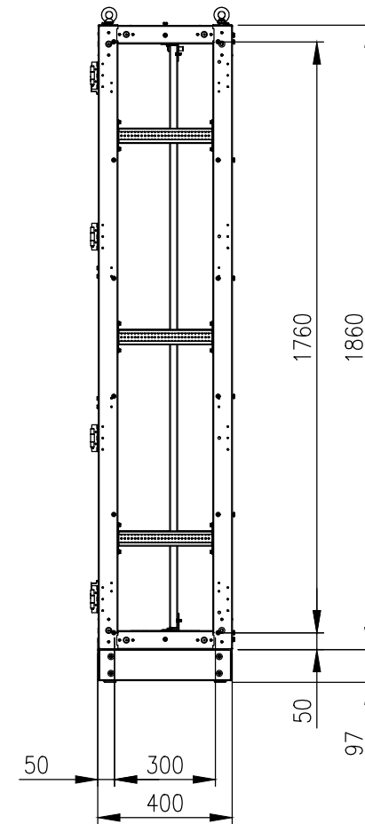
SIDE VIEW (PANELS REMOVED)
