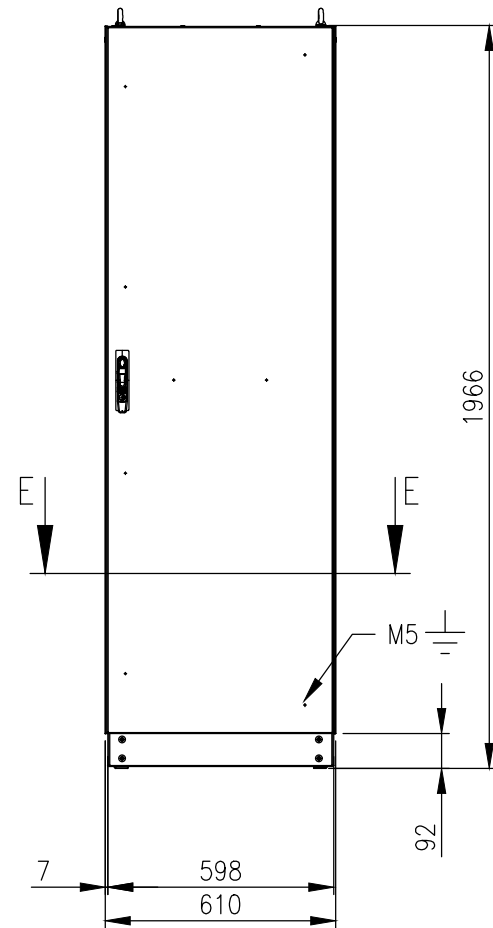
FRONT VIEW (ASSEMBLY)
