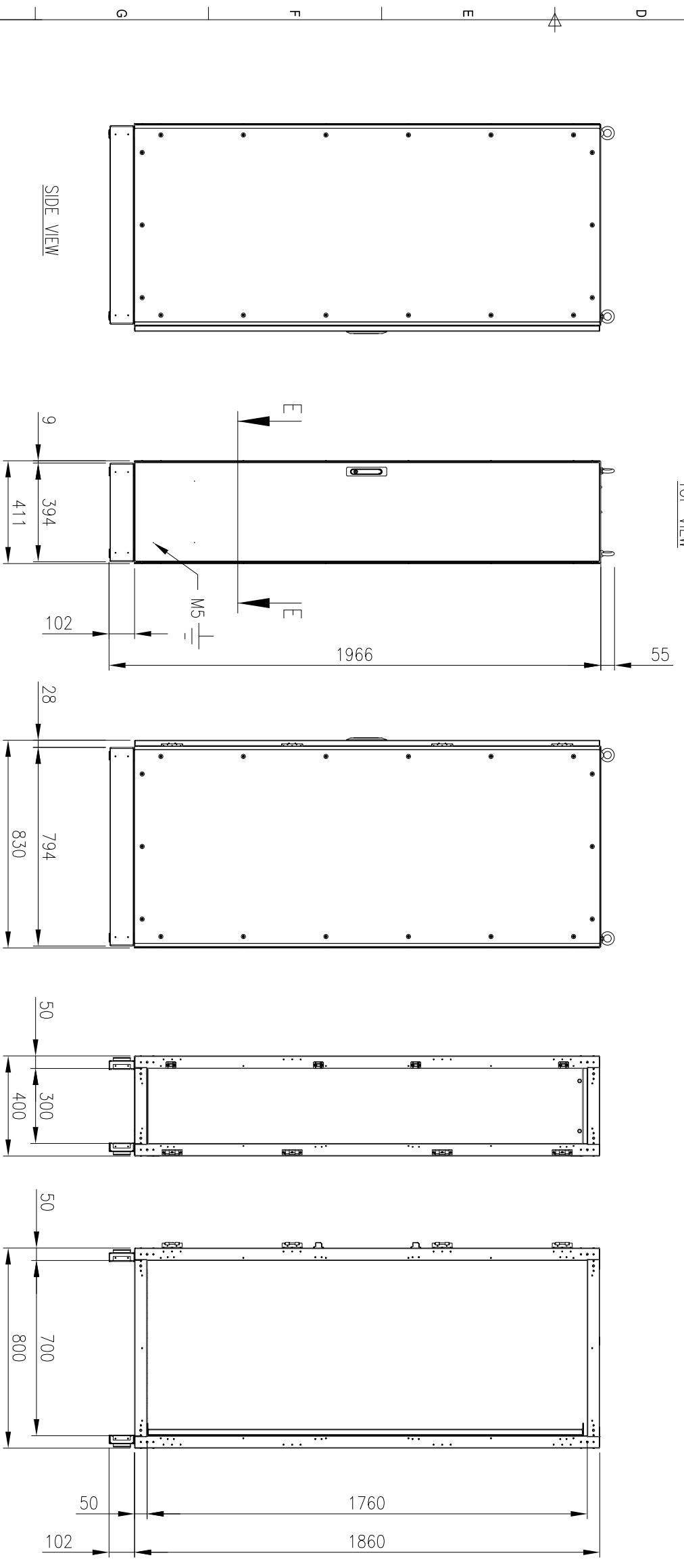
SIDE VIEW
