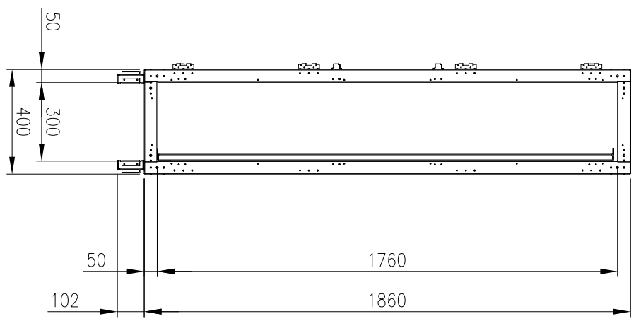
SIDE VIEW (PANELS REMOVED)
