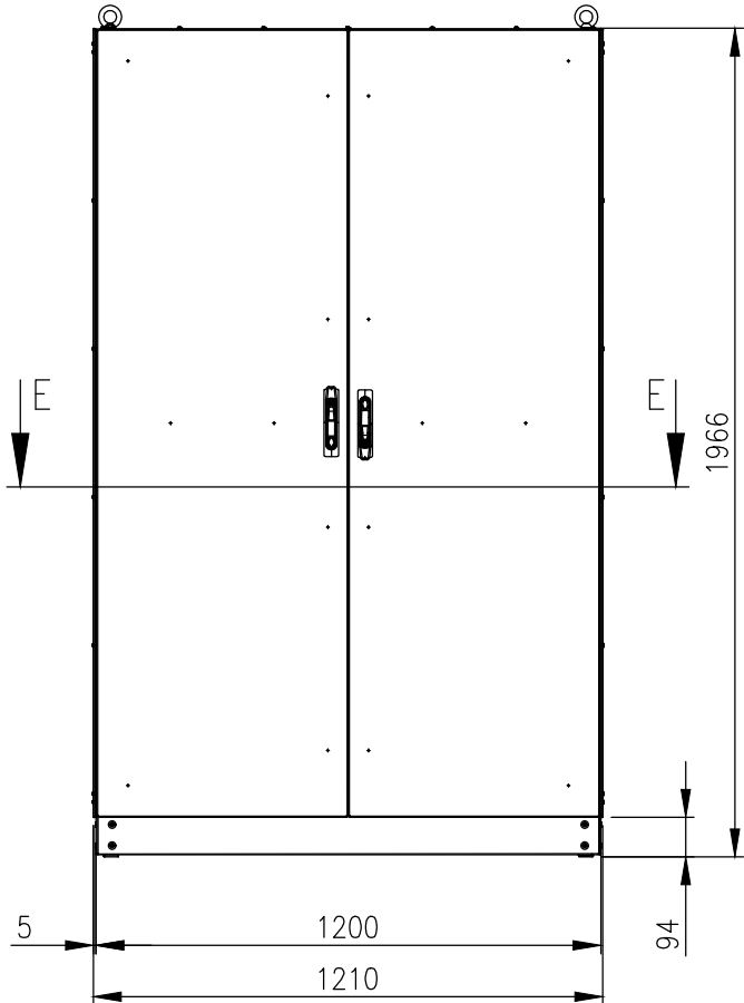
FRONT VIEW (ASSEMBLY)
