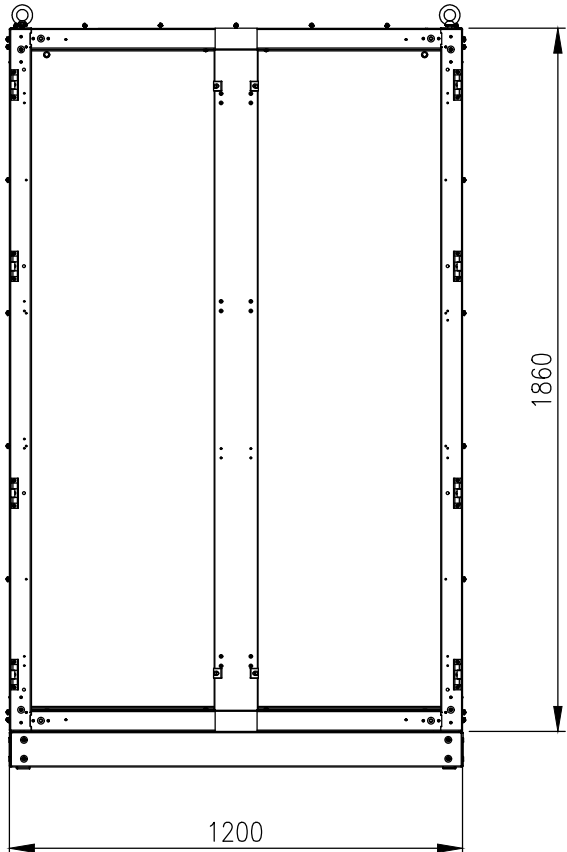
FRONT VIEW (PANELS REMOVED)
