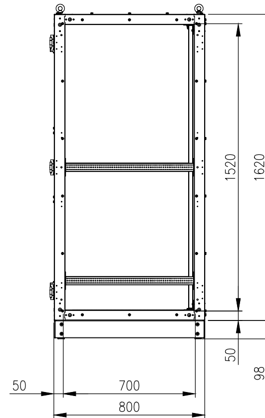
SIDE VIEW (PANELS REMOVED)
