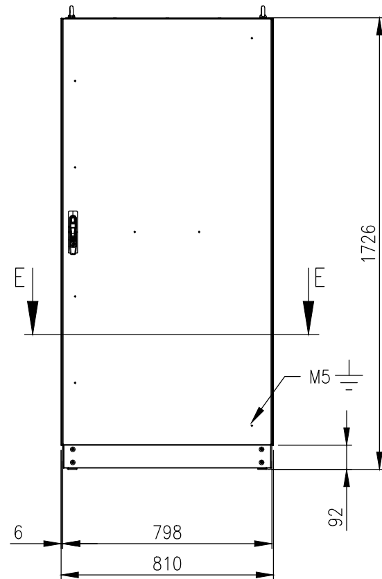
FRONT VIEW (ASSEMBLY)
