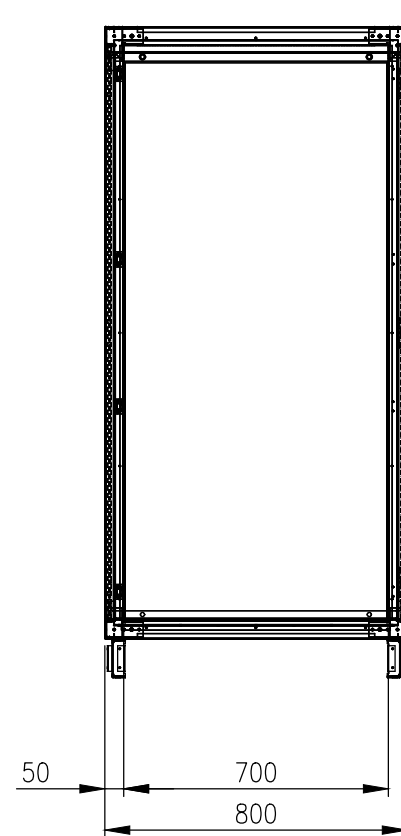
FRONT VIEW (PANELS REMOVED)
