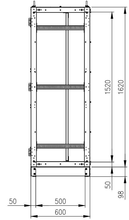
SIDE VIEW (PANELS REMOVED)
