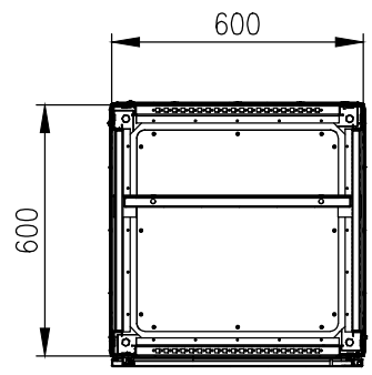
SECTION E-E
