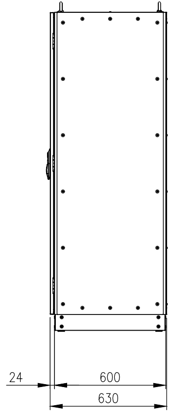
SIDE VIEW
