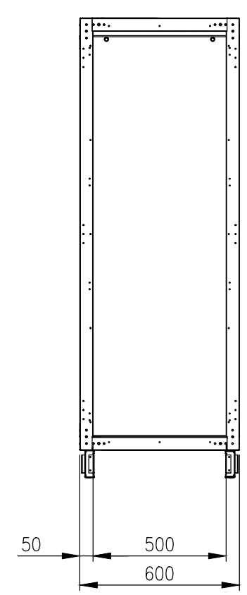
FRONT VIEW (PANELS REMOVED)
