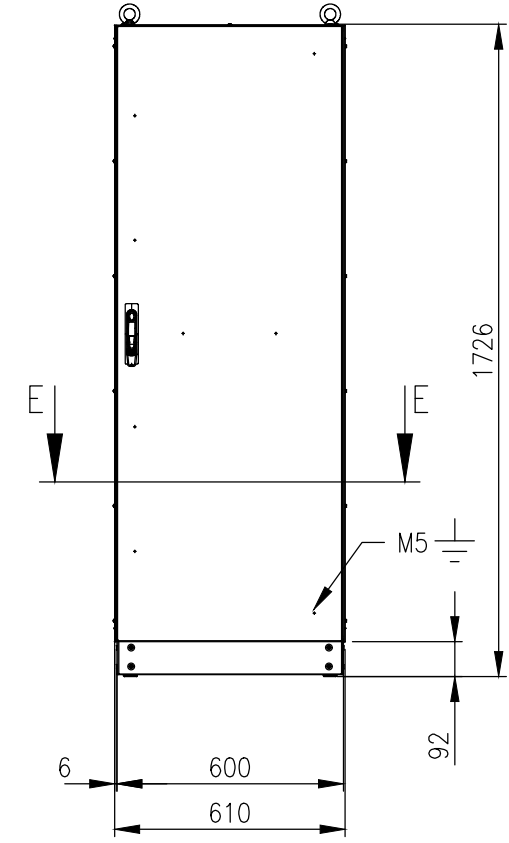
FRONT VIEW (ASSEMBLY)
