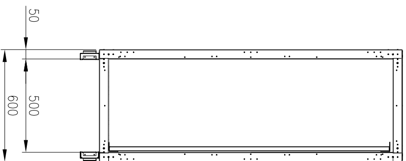
SIDE VIEW (PANELS REMOVED)
