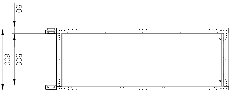
FRONT VIEW (PANELS REMOVED)
