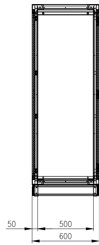
FRONT VIEW (PANELS REMOVED)
