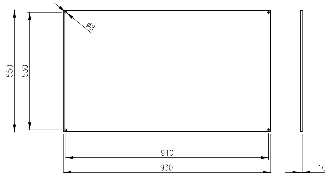
DEVICE MOUNTING PLATE
