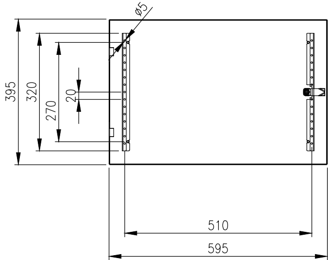
INSIDE DOOR VIEW
