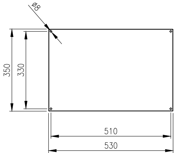
DEVICE MOUNTING PLATE
