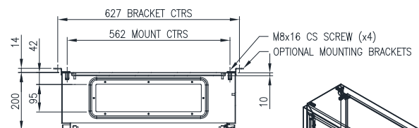
SECTION AW-AW
