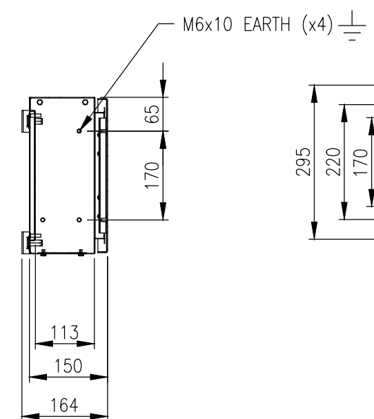
SECTION AW-AW
