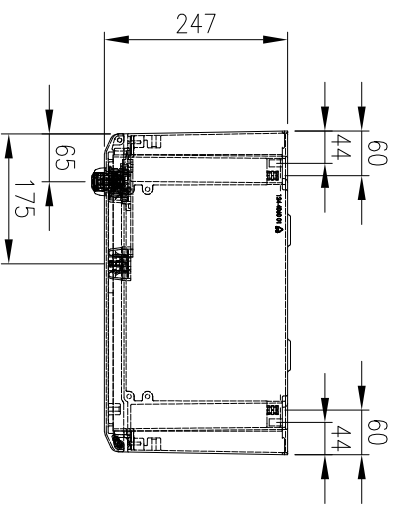
SECTION AW-AW
