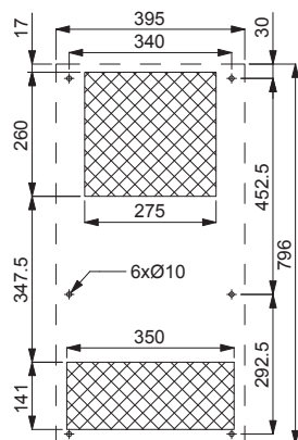
MOUNTING CUT-OUT
