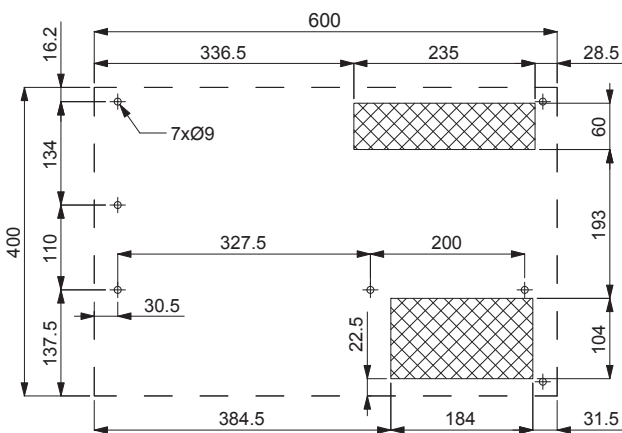
MOUNTING CUT-OUT
