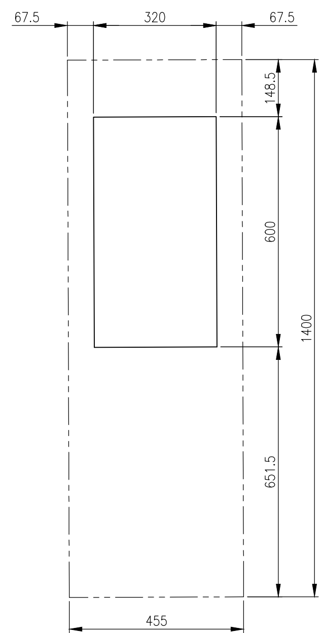
MOUNTING CUT-OUT
