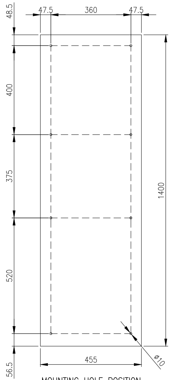
MOUNTING HOLE POSITION
