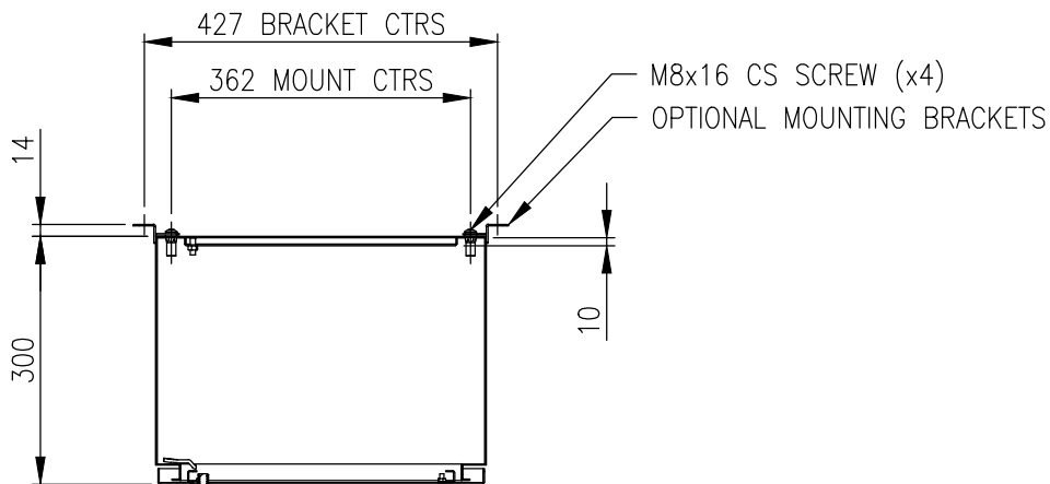
SECTION AW-AW
