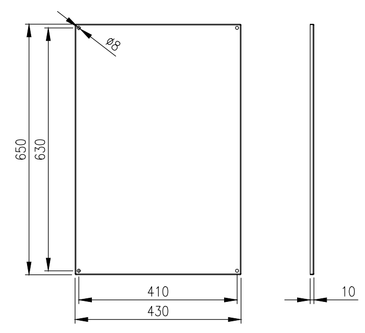
DEVICE MOUNTING PLATE
