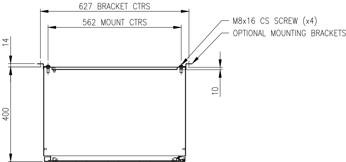
SECTION AW-AW
