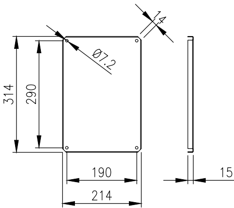
DEVICE MOUNTING PLATE
