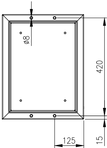
REAR VIEW
