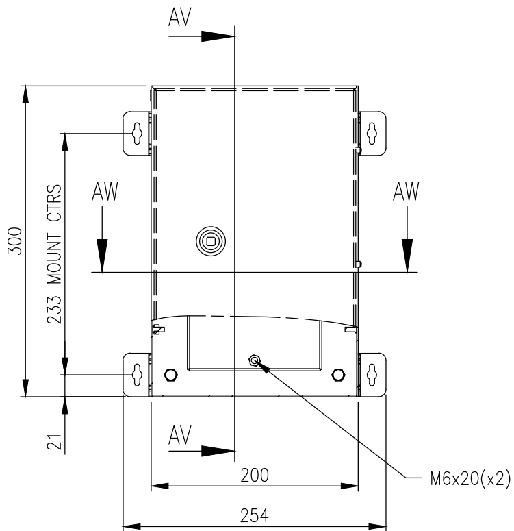
FRONT VIEW
