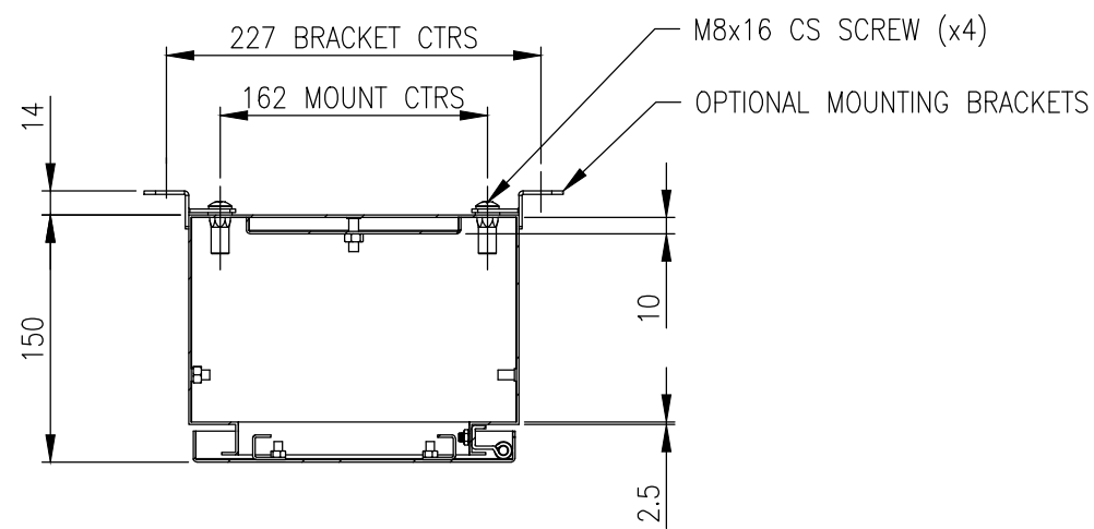
SECTION AW-AW
