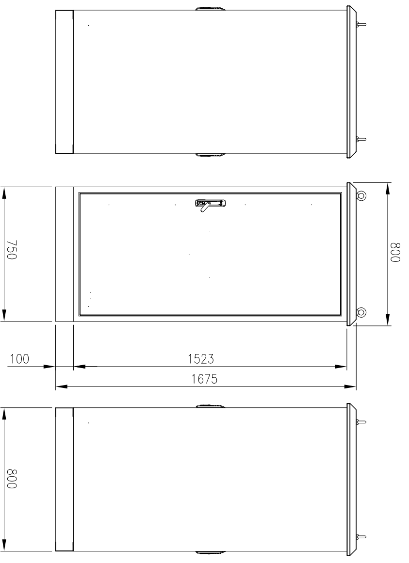
SIDE VIEW
