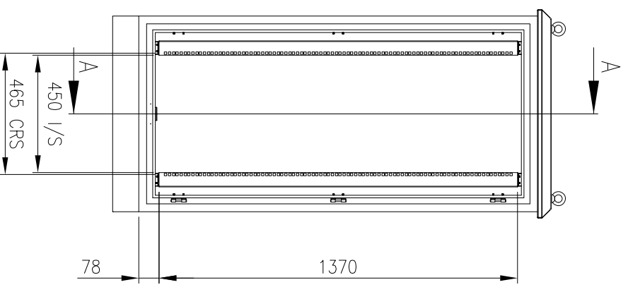
FRONT VIEW (FRONT DOOR REMOVED)
