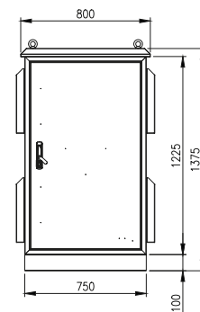
FRONT VIEW (ASSEMBLY)
