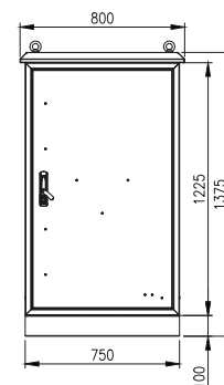
FRONT VIEW (ASSEMBLY)
