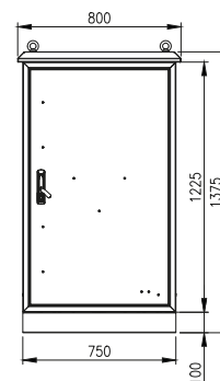
FRONT VIEW (ASSEMBLY)
